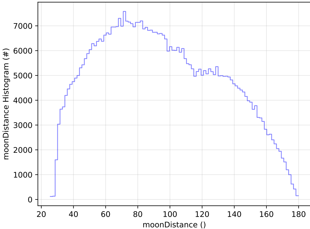
early_u_fpextra2.0_v3.4_10yrs All sky i band: moonDistance Histogram
