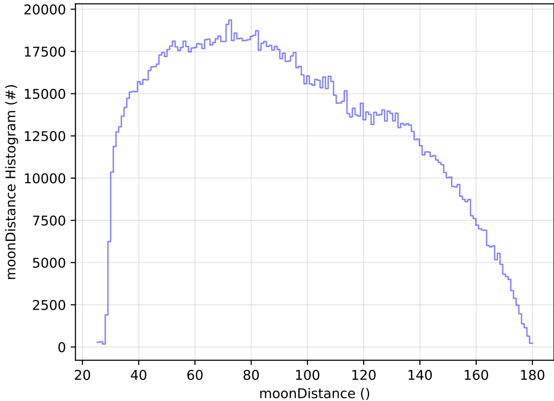
early_u_fpextra2.0_v3.4_10yrs All sky all bands: moonDistance Histogram
