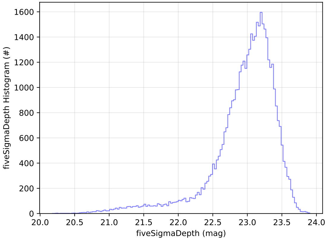
early_u_fpextra2.0_v3.4_10yrs Yr 1 z band: fiveSigmaDepth Histogram
