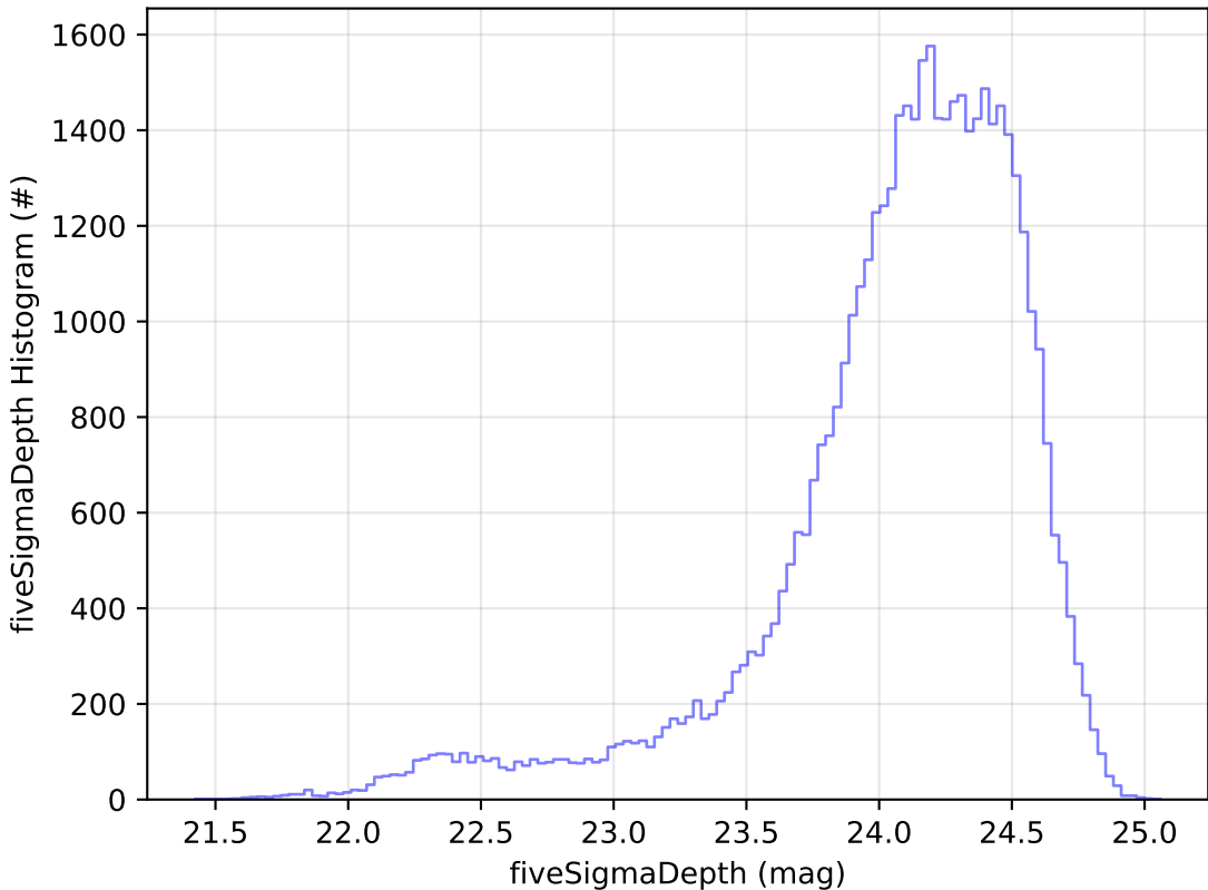
early_u_fpextra2.0_v3.4_10yrs Yr 1 r band: fiveSigmaDepth Histogram
