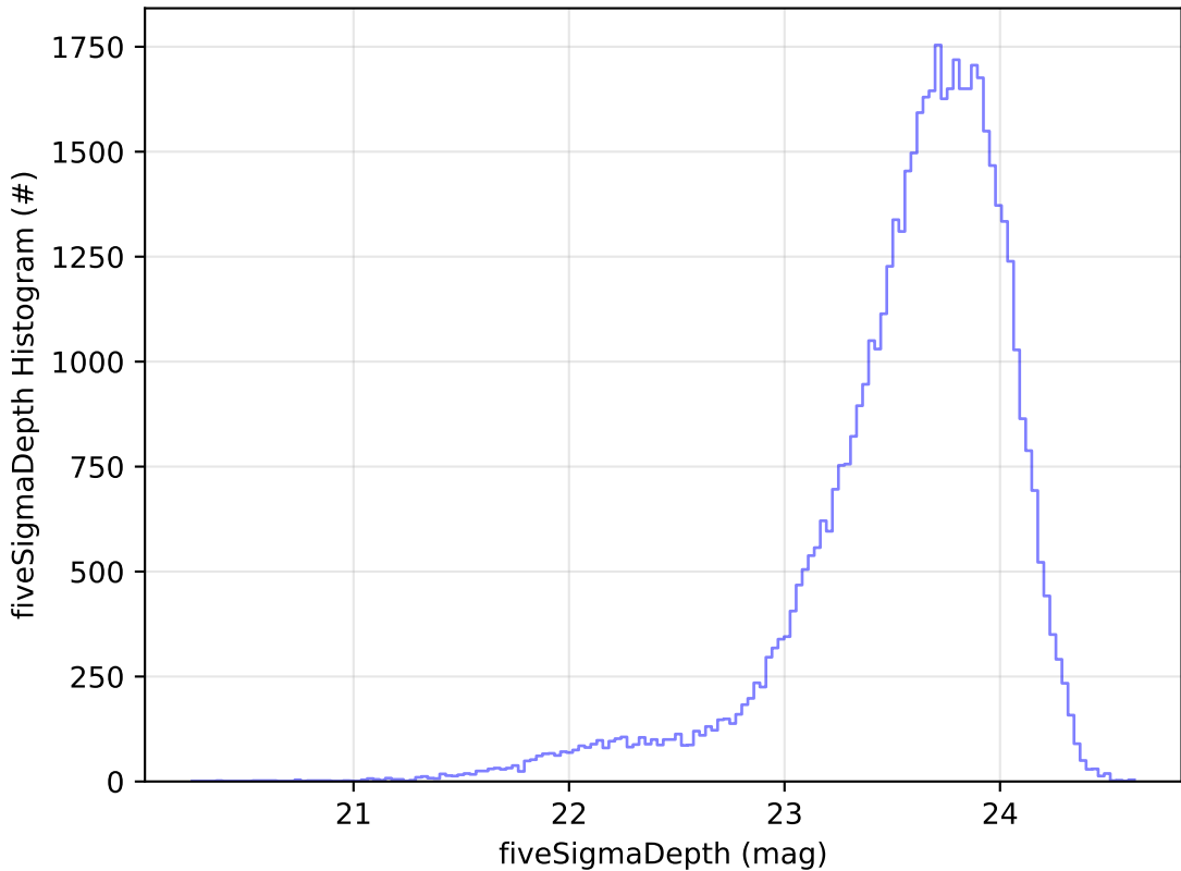
early_u_fpextra2.0_v3.4_10yrs Yr 1 i band: fiveSigmaDepth Histogram
