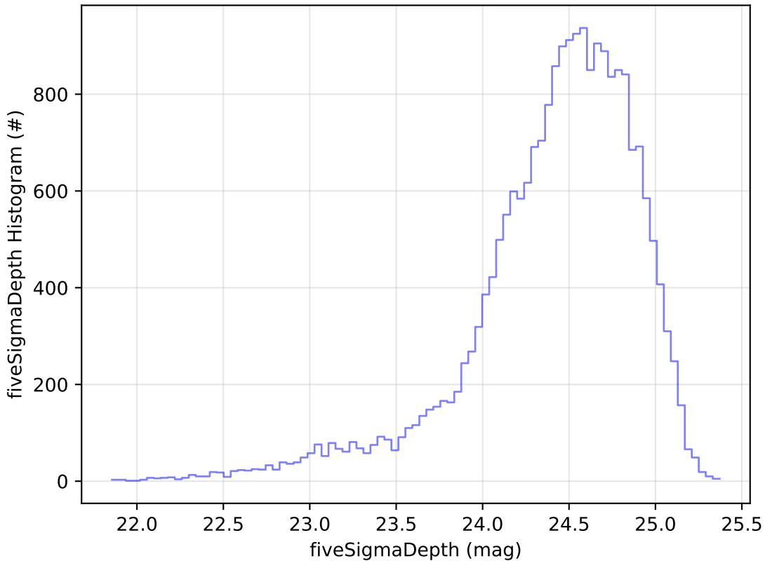
early_u_fpextra2.0_v3.4_10yrs Yr 1 g band: fiveSigmaDepth Histogram
