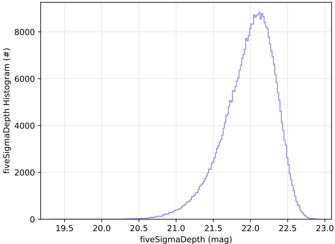
early_u_fpextra2.0_v3.4_10yrs WFD y band: fiveSigmaDepth Histogram
