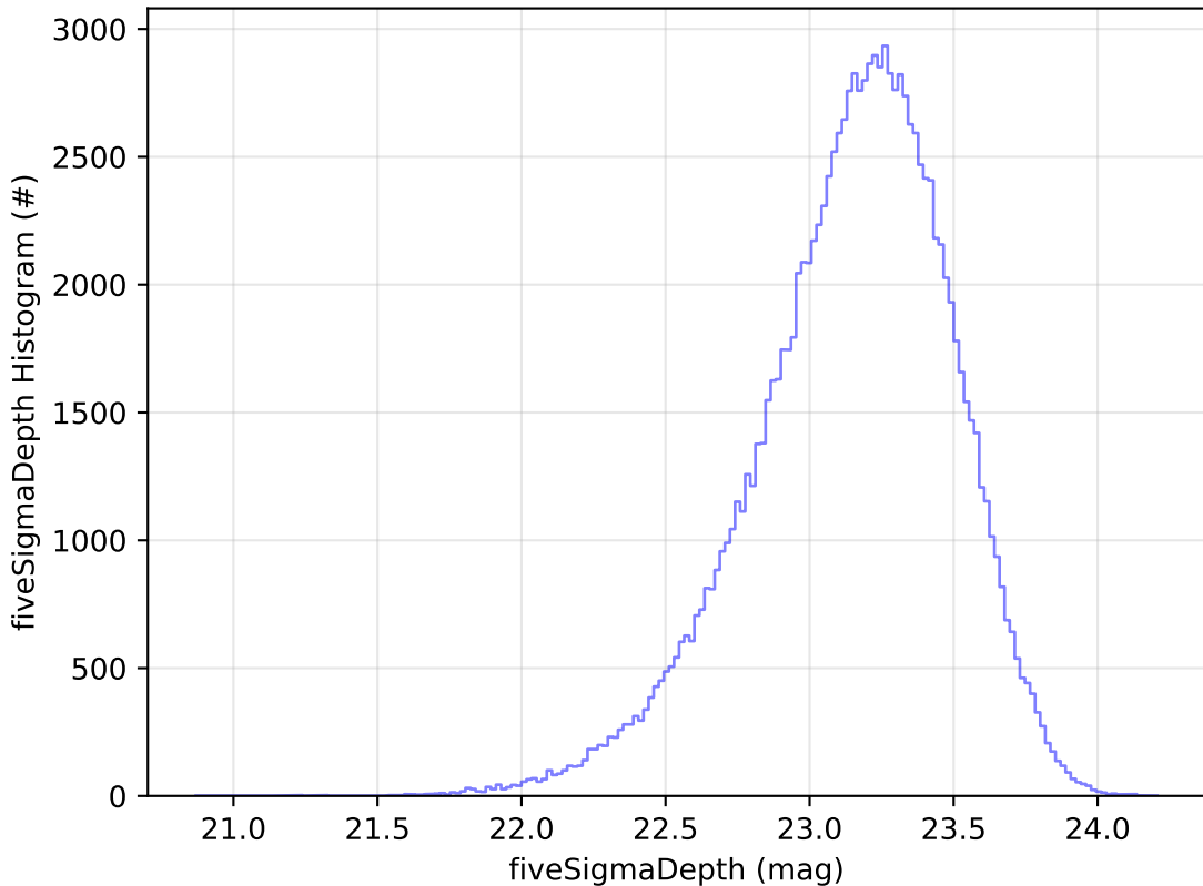
early_u_fpextra2.0_v3.4_10yrs WFD u band: fiveSigmaDepth Histogram
