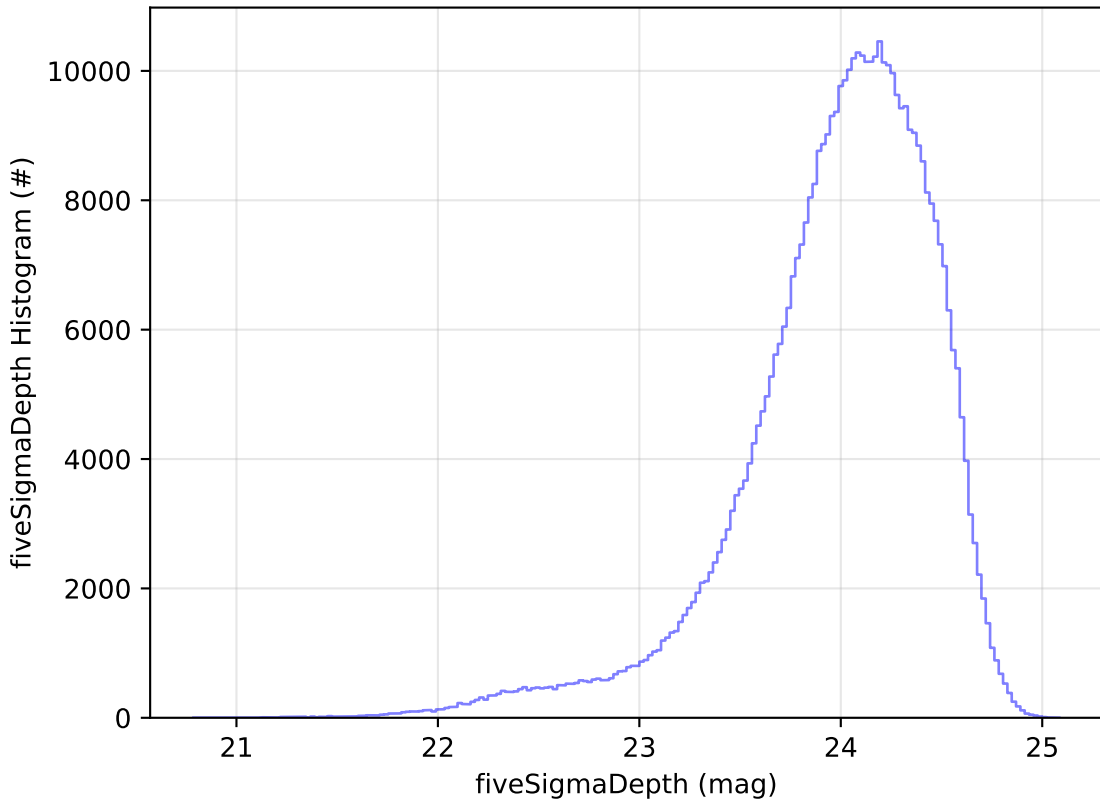
early_u_fpextra2.0_v3.4_10yrs WFD r band: fiveSigmaDepth Histogram
