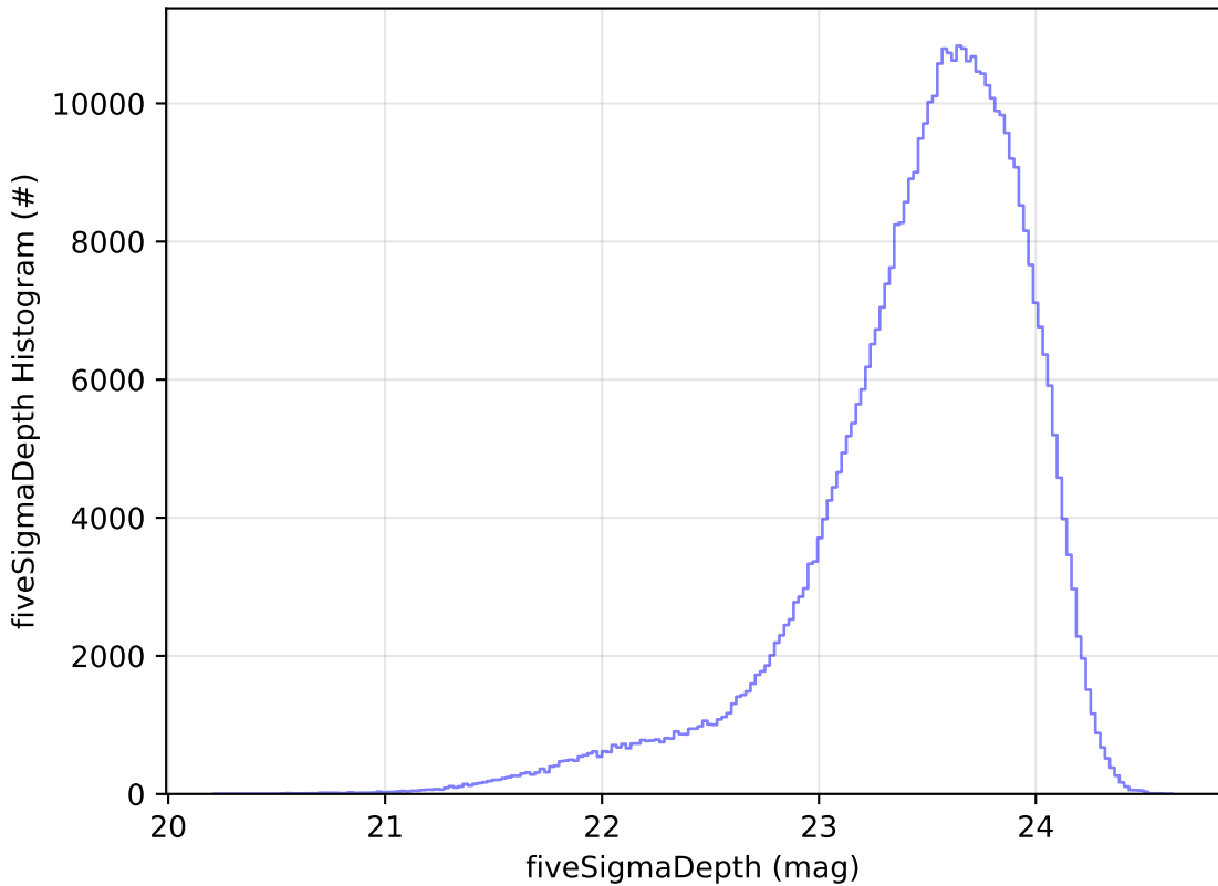
early_u_fpextra2.0_v3.4_10yrs WFD i band: fiveSigmaDepth Histogram
