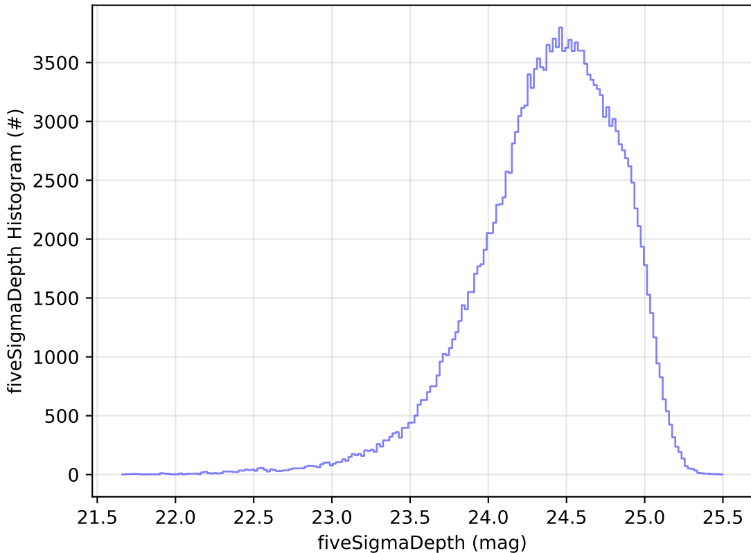
early_u_fpextra2.0_v3.4_10yrs WFD g band: fiveSigmaDepth Histogram
