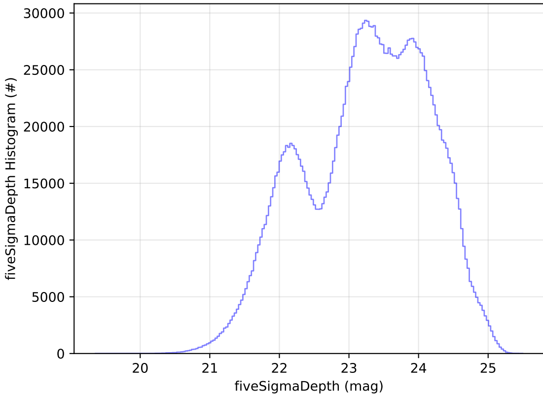
early_u_fpextra2.0_v3.4_10yrs WFD all bands: fiveSigmaDepth Histogram
