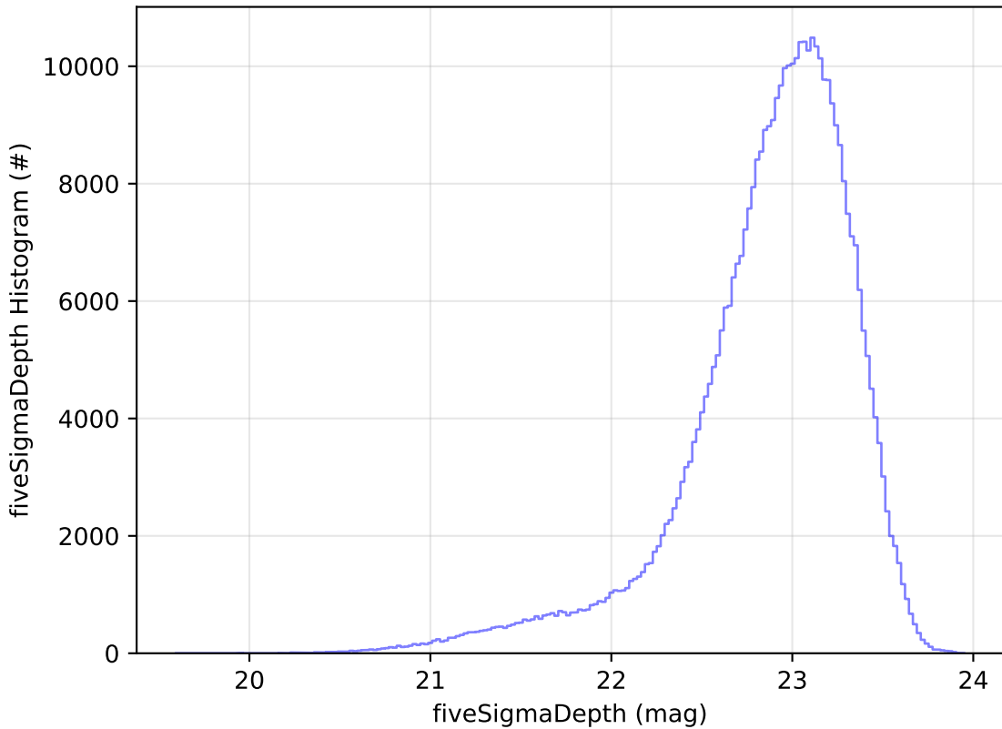
early_u_fpextra2.0_v3.4_10yrs All sky z band: fiveSigmaDepth Histogram
