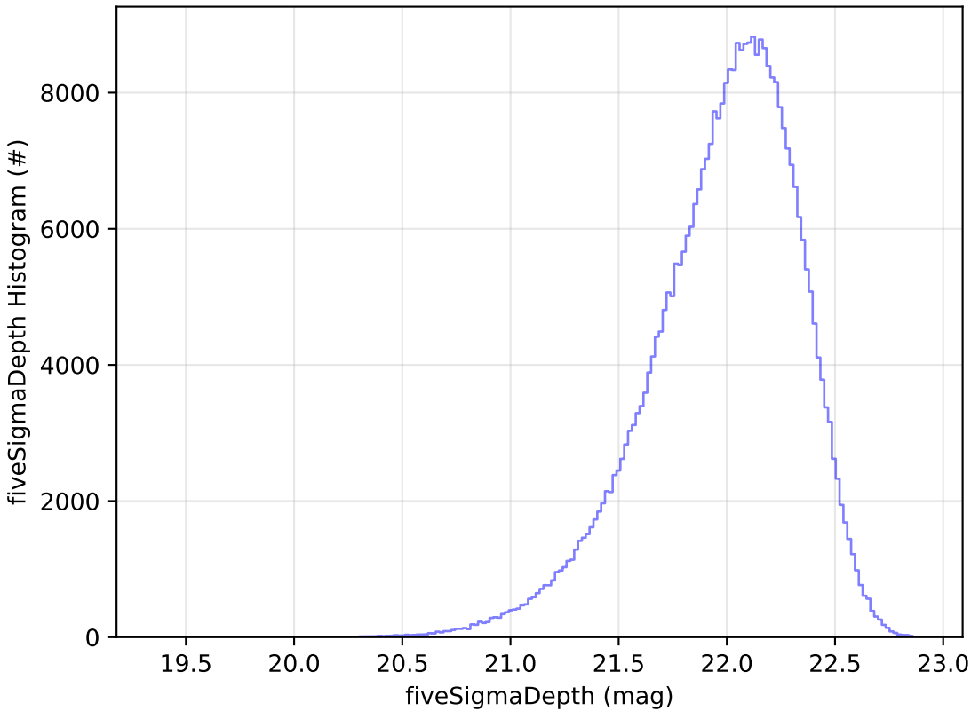
early_u_fpextra2.0_v3.4_10yrs All sky y band: fiveSigmaDepth Histogram
