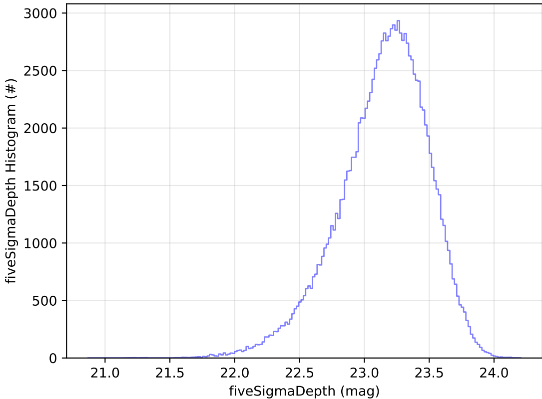
early_u_fpextra2.0_v3.4_10yrs All sky u band: fiveSigmaDepth Histogram
