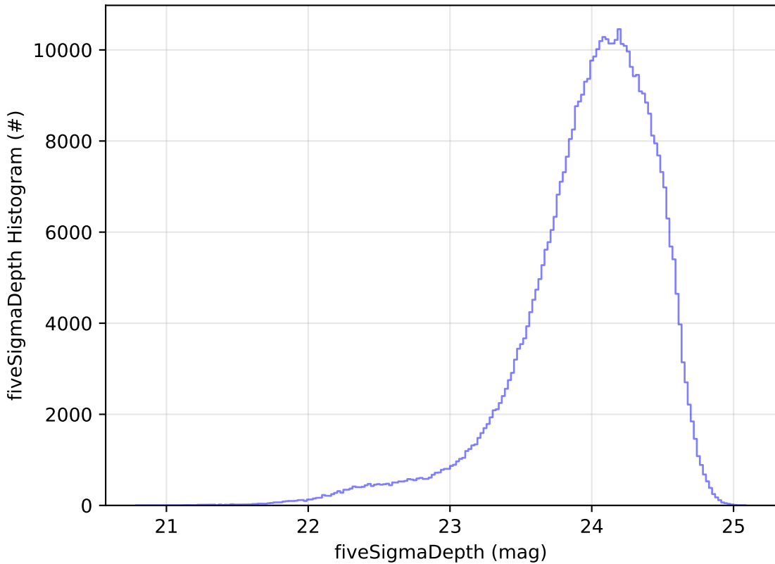
early_u_fpextra2.0_v3.4_10yrs All sky r band: fiveSigmaDepth Histogram
