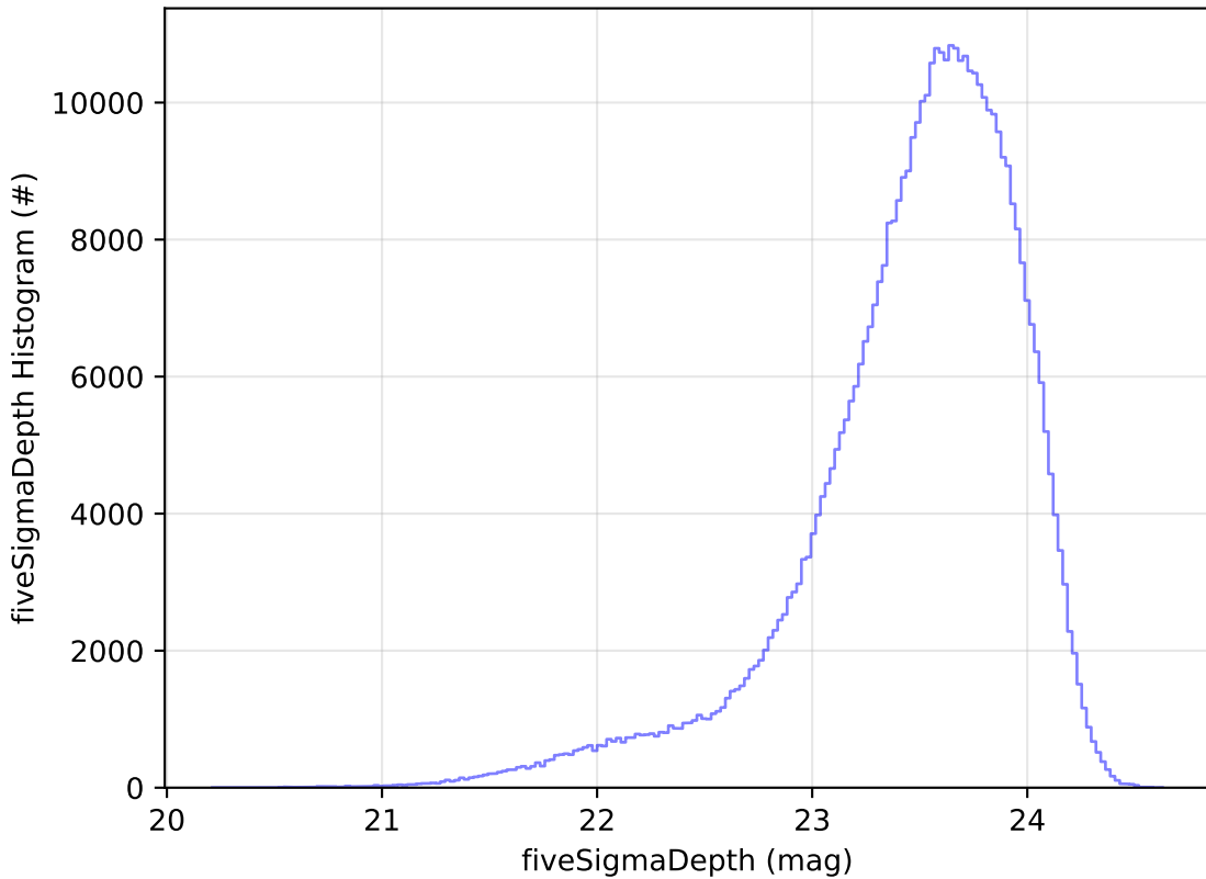
early_u_fpextra2.0_v3.4_10yrs All sky i band: fiveSigmaDepth Histogram
