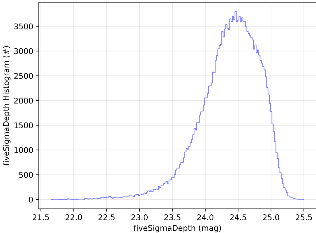
early_u_fpextra2.0_v3.4_10yrs All sky g band: fiveSigmaDepth Histogram
