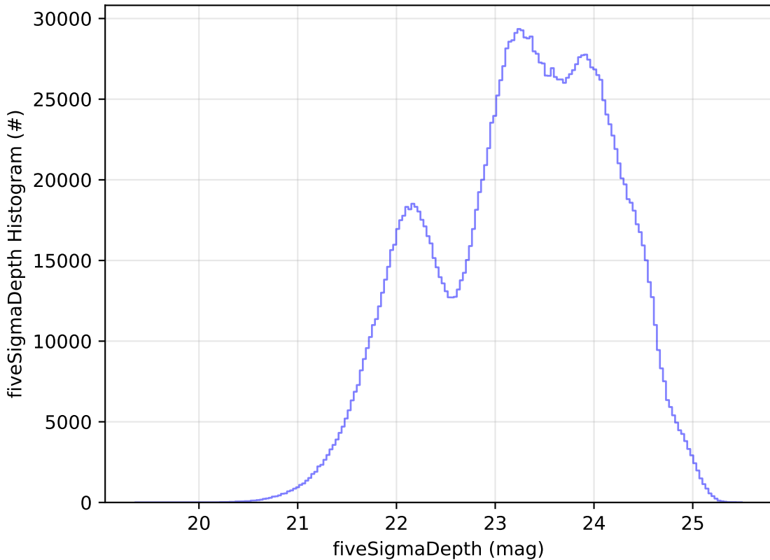
early_u_fpextra2.0_v3.4_10yrs All sky all bands: fiveSigmaDepth Histogram
