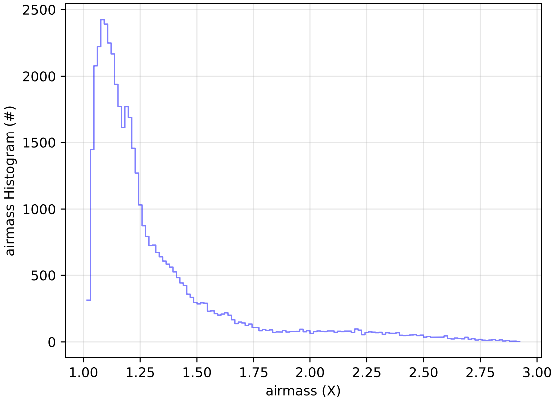
early_u_fpextra2.0_v3.4_10yrs Yr 1 z band: airmass Histogram
