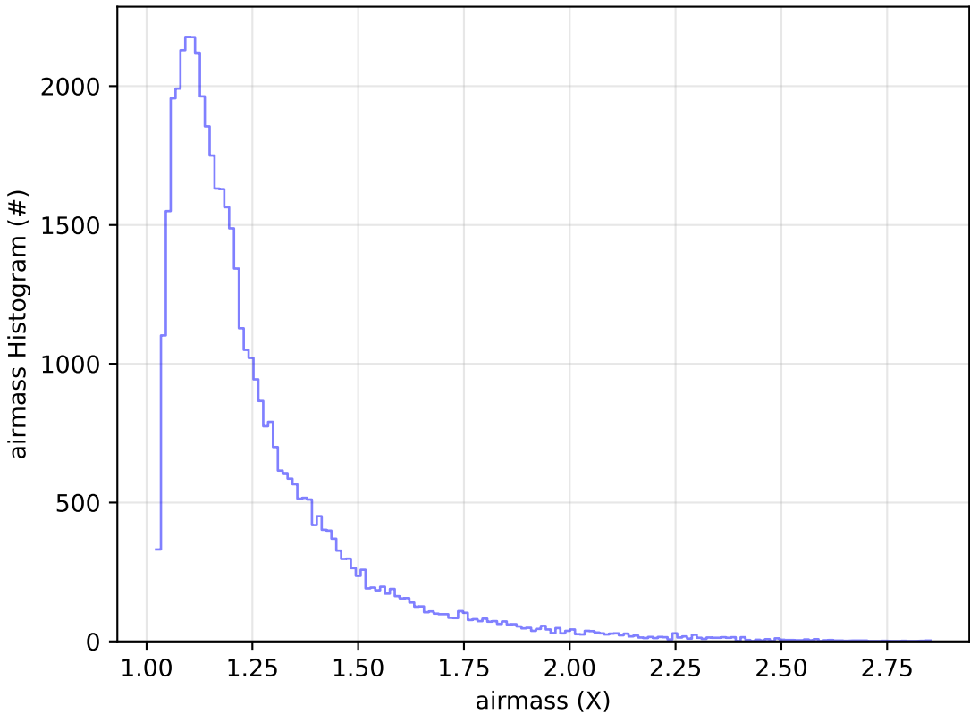
early_u_fpextra2.0_v3.4_10yrs Yr 1 y band: airmass Histogram
