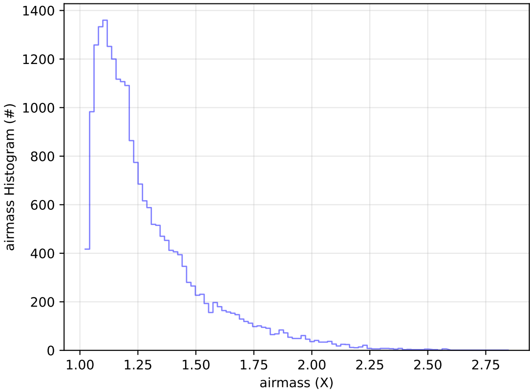
early_u_fpextra2.0_v3.4_10yrs Yr 1 u band: airmass Histogram
