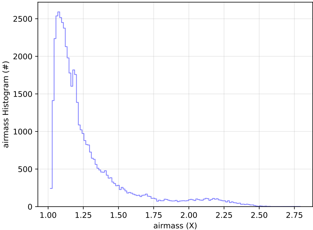
early_u_fpextra2.0_v3.4_10yrs Yr 1 r band: airmass Histogram
