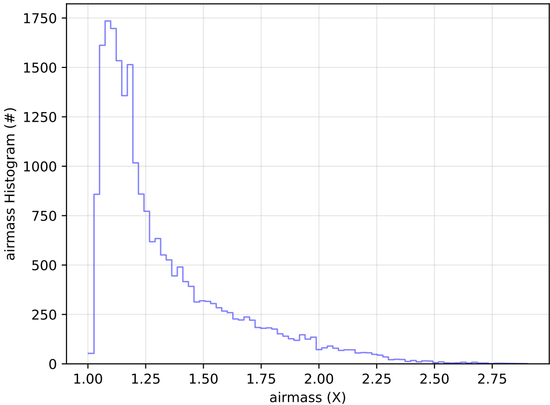
early_u_fpextra2.0_v3.4_10yrs Yr 1 g band: airmass Histogram
