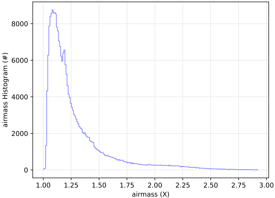
early_u_fpextra2.0_v3.4_10yrs Yr 1 all bands: airmass Histogram
