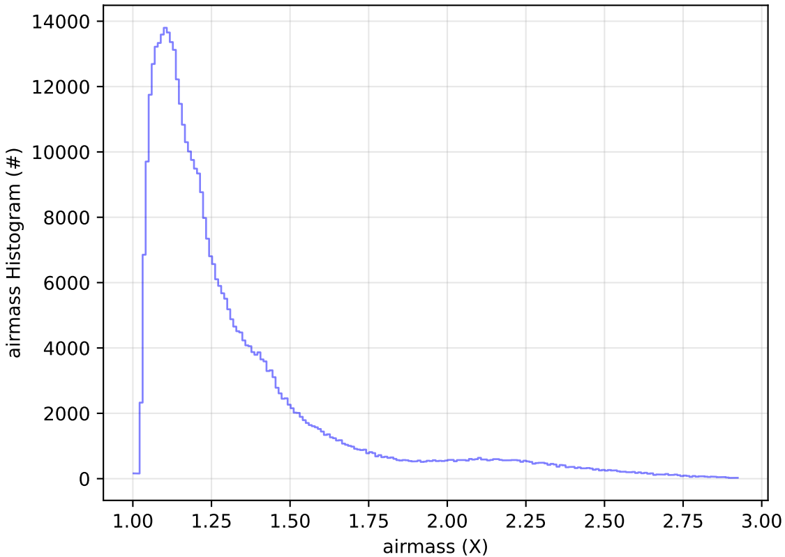
early_u_fpextra2.0_v3.4_10yrs WFD z band: airmass Histogram
