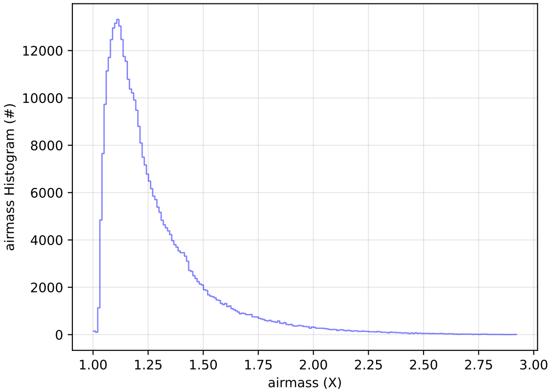
early_u_fpextra2.0_v3.4_10yrs WFD y band: airmass Histogram
