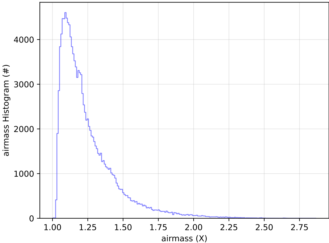
early_u_fpextra2.0_v3.4_10yrs WFD u band: airmass Histogram
