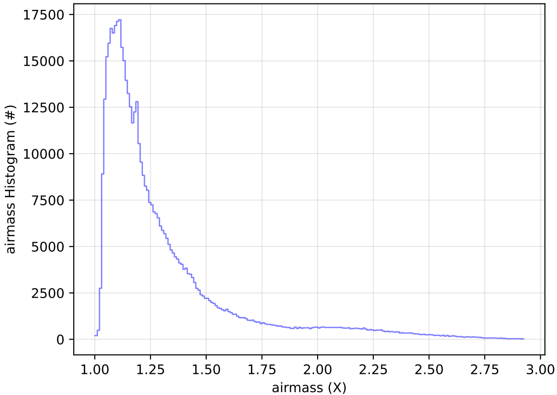
early_u_fpextra2.0_v3.4_10yrs WFD i band: airmass Histogram
