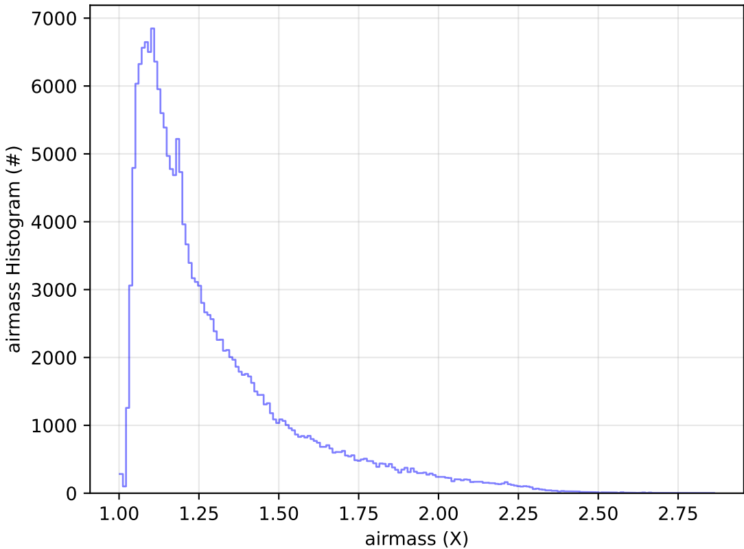
early_u_fpextra2.0_v3.4_10yrs WFD g band: airmass Histogram
