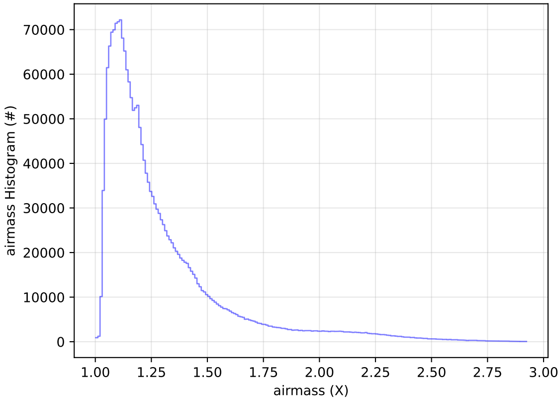
early_u_fpextra2.0_v3.4_10yrs WFD all bands: airmass Histogram
