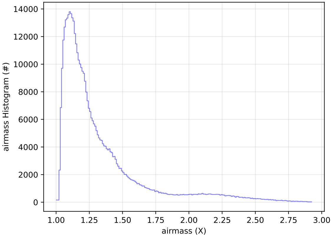
early_u_fpextra2.0_v3.4_10yrs All sky z band: airmass Histogram
