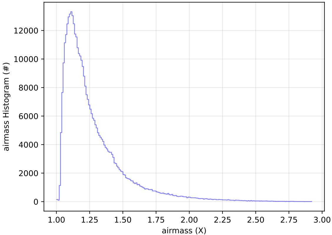
early_u_fpextra2.0_v3.4_10yrs All sky y band: airmass Histogram
