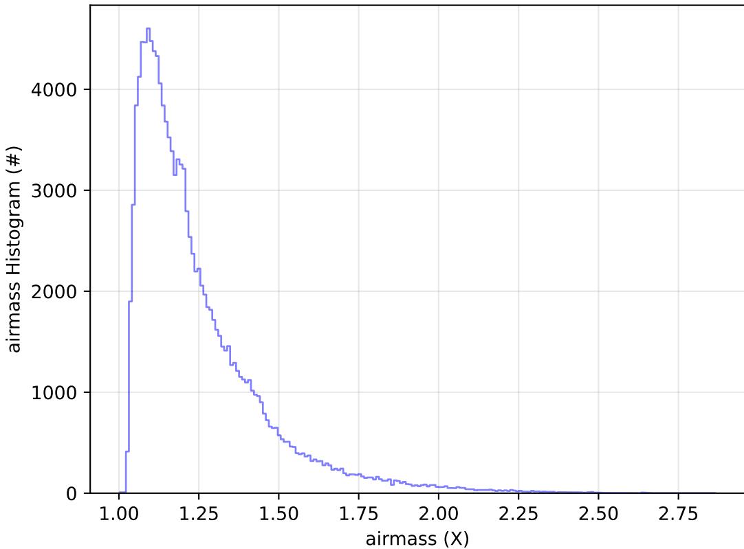
early_u_fpextra2.0_v3.4_10yrs All sky u band: airmass Histogram
