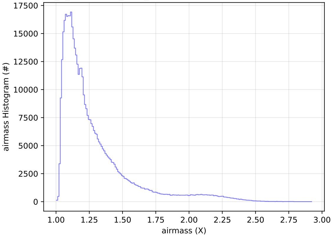
early_u_fpextra2.0_v3.4_10yrs All sky r band: airmass Histogram
