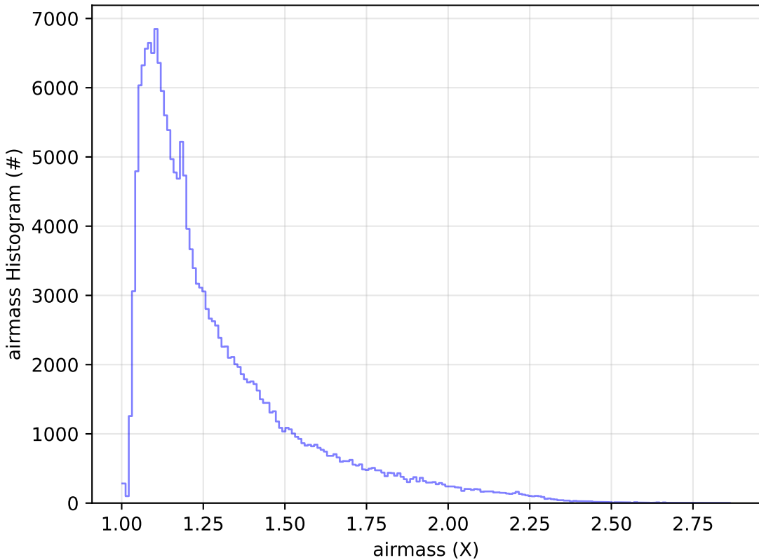
early_u_fpextra2.0_v3.4_10yrs All sky g band: airmass Histogram
