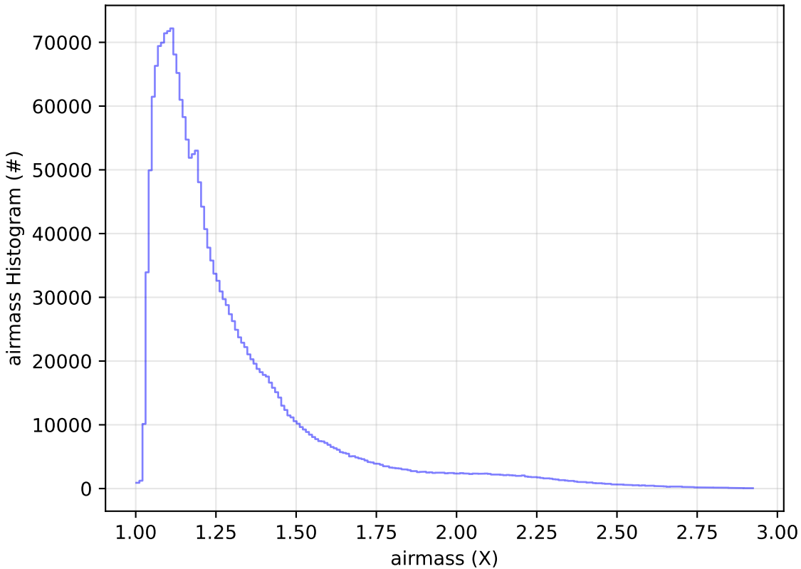
early_u_fpextra2.0_v3.4_10yrs All sky all bands: airmass Histogram
