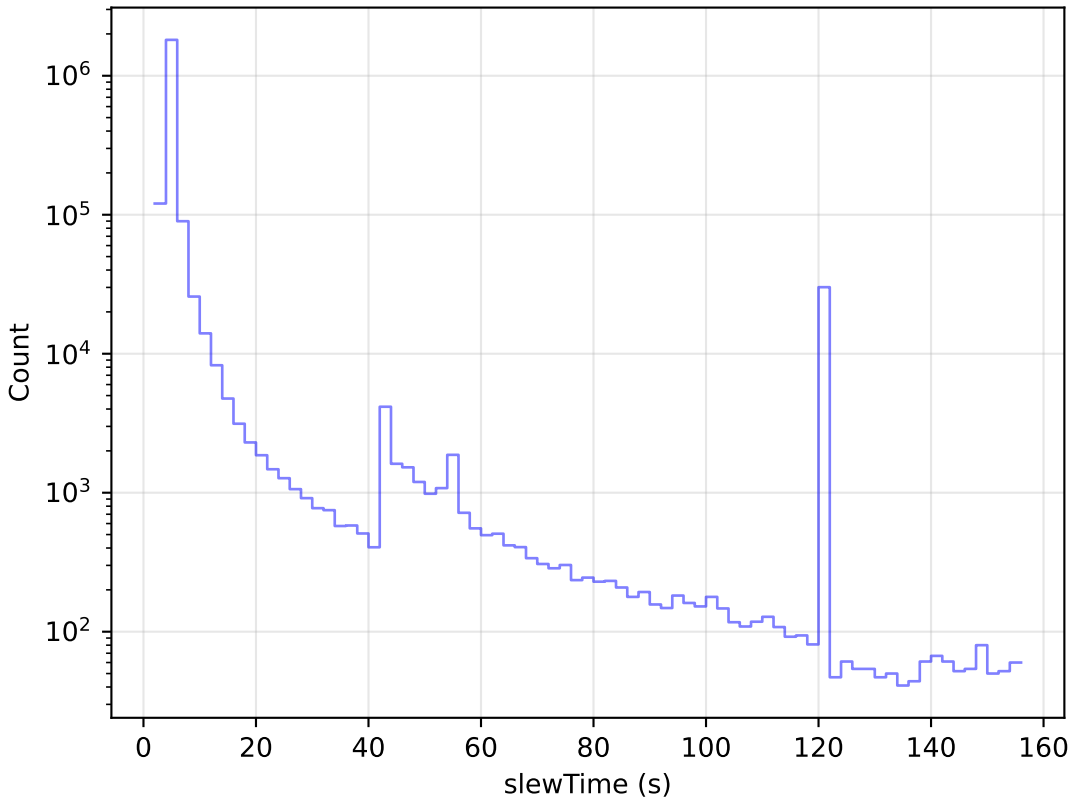
early_u_fpextra2.0_v3.4_10yrs All visits: Slew Time Histogram
