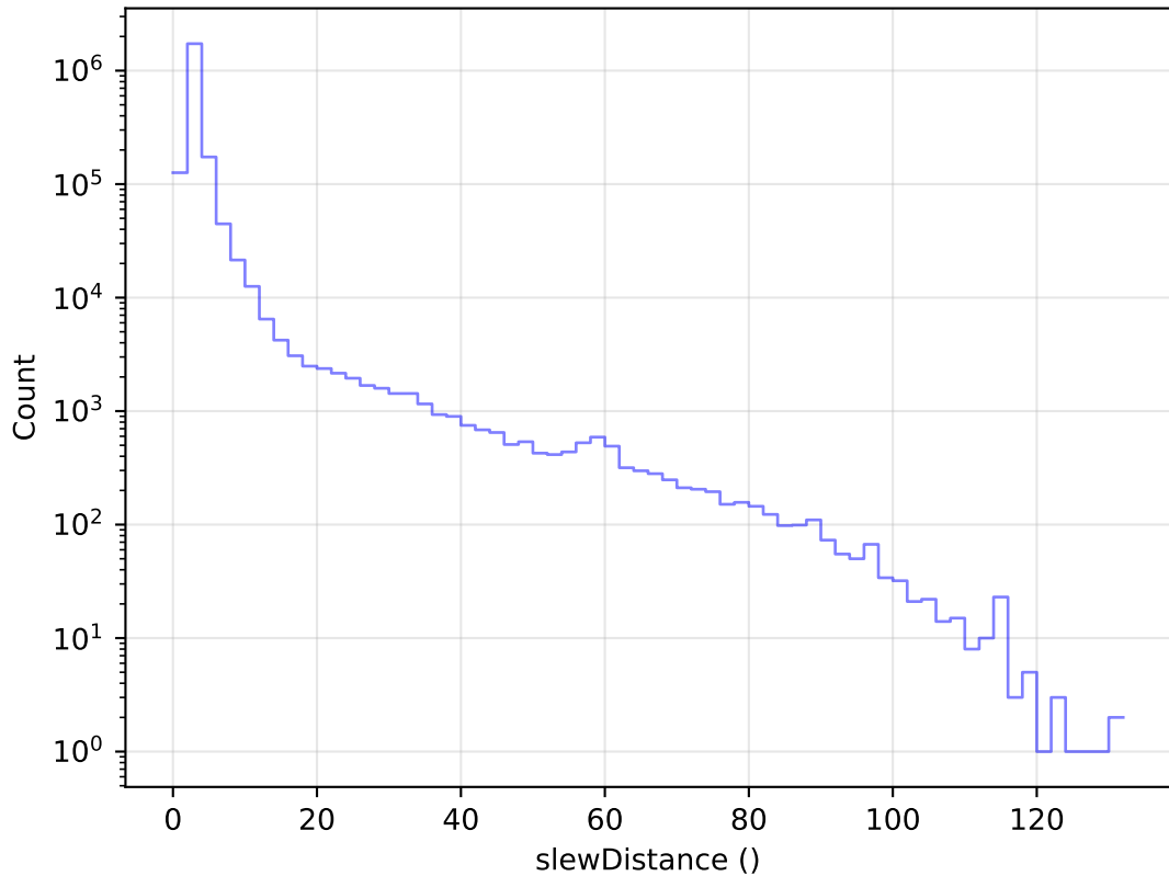
early_u_fpextra2.0_v3.4_10yrs All visits: Slew Distance Histogram
