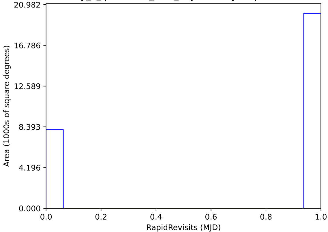
early_u_fpextra2.0_v3.4_10yrs All sky: RapidRevisits
