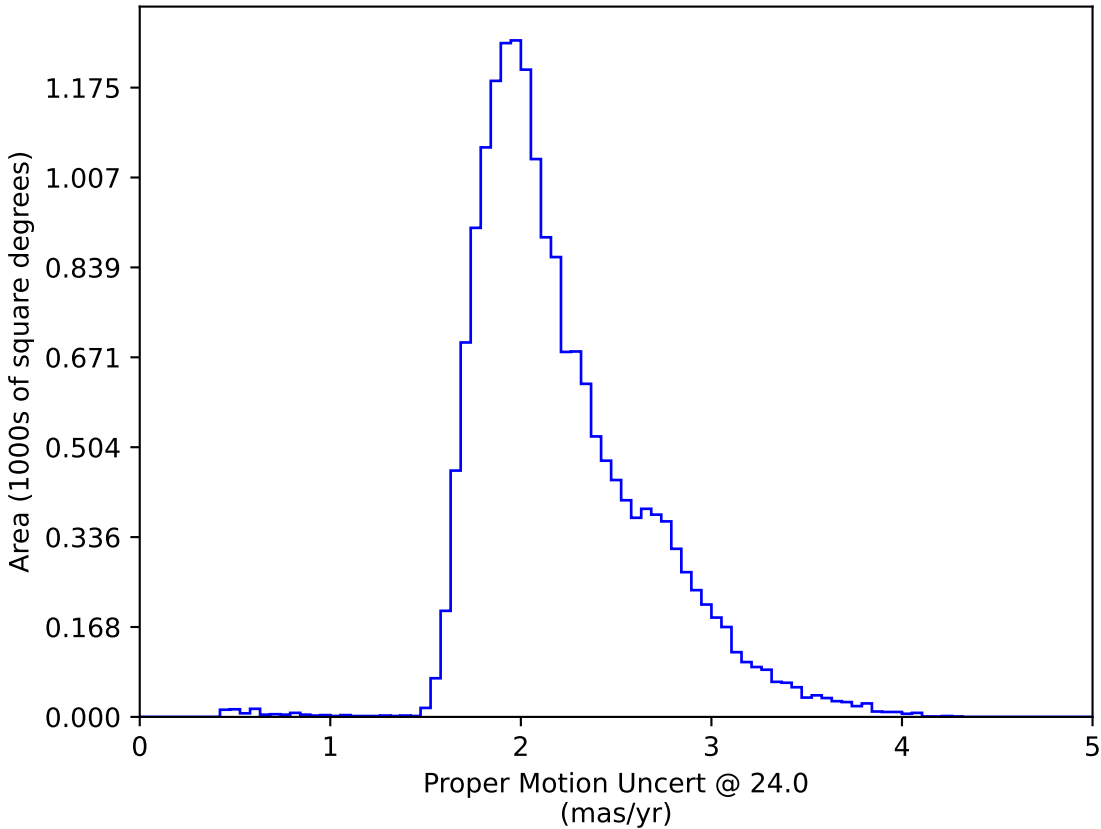
early_u_fpextra2.0_v3.4_10yrs WFD: Proper Motion Uncert @ 24.0
