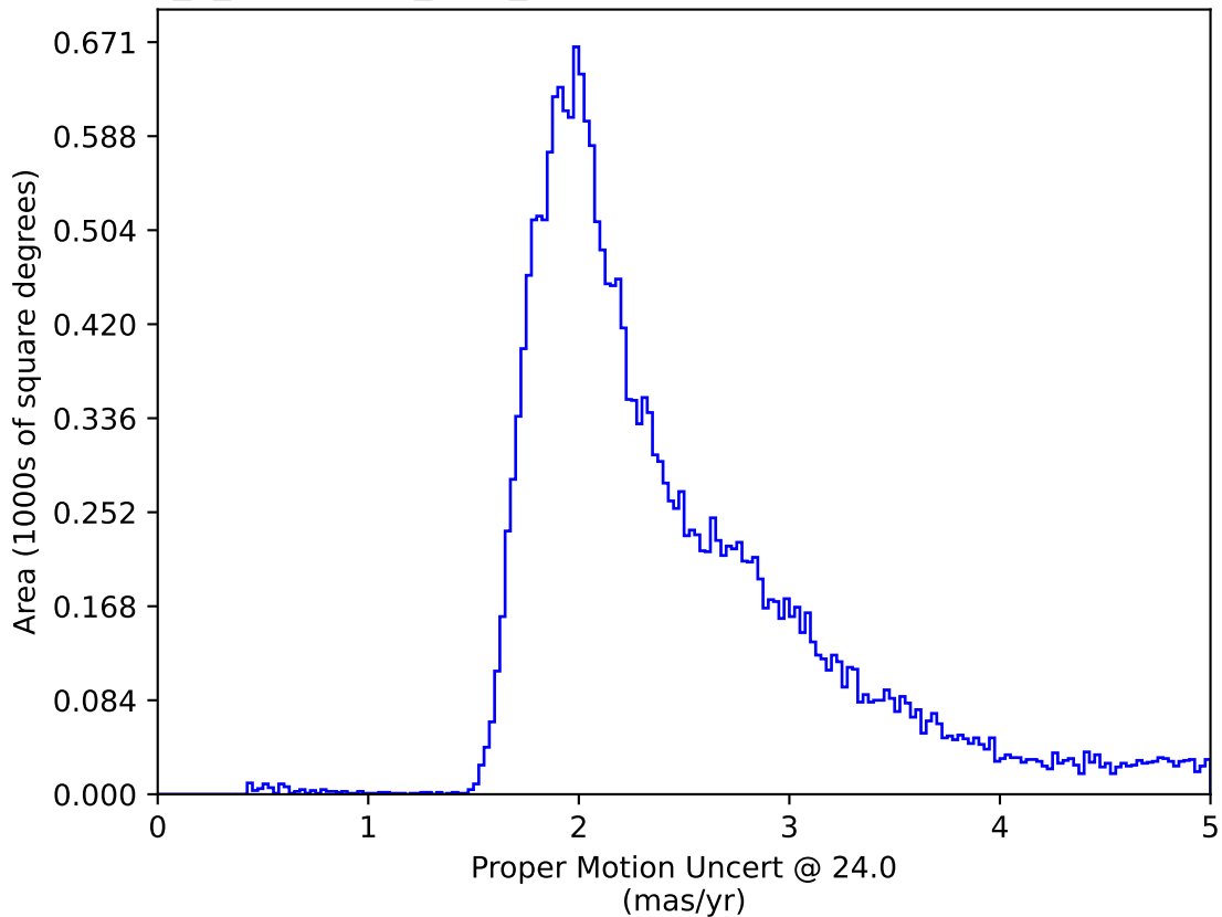
early_u_fpextra2.0_v3.4_10yrs All sky: Proper Motion Uncert @ 24.0
