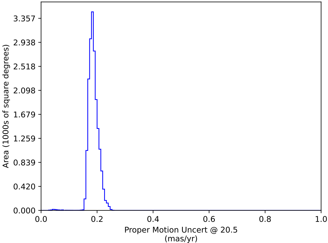
early_u_fpextra2.0_v3.4_10yrs WFD: Proper Motion Uncert @ 20.5
