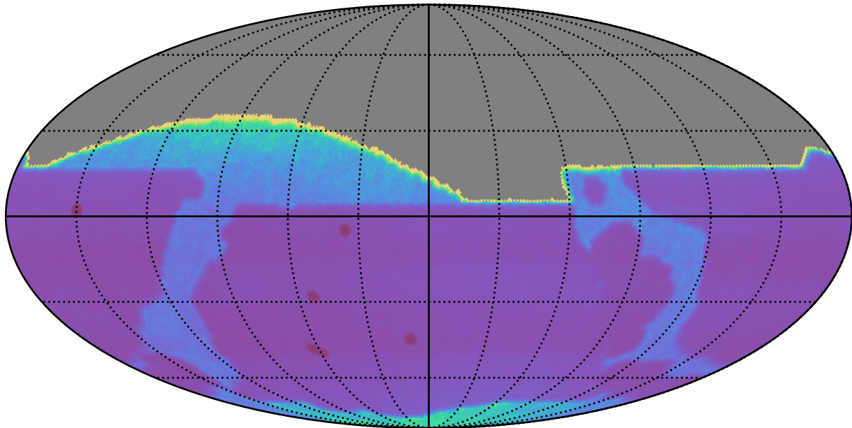
early_u_fpextra2.0_v3.4_10yrs All sky: Proper Motion Uncert @ 20.5
