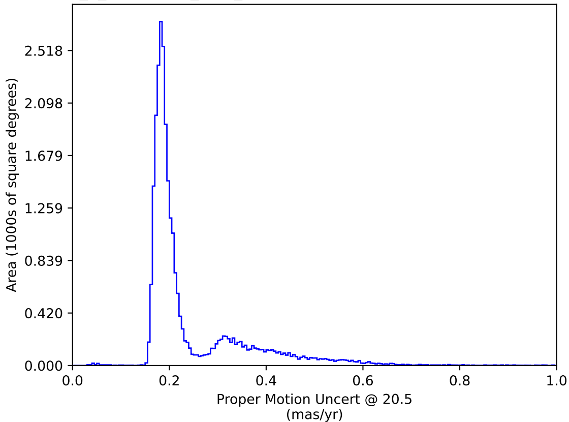
early_u_fpextra2.0_v3.4_10yrs All sky: Proper Motion Uncert @ 20.5
