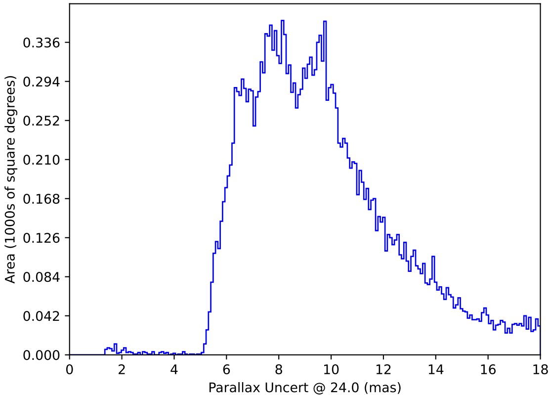
early_u_fpextra2.0_v3.4_10yrs All sky: Parallax Uncert @ 24.0
