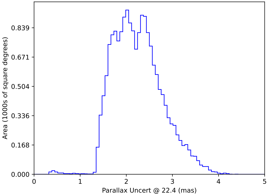
early_u_fpextra2.0_v3.4_10yrs WFD: Parallax Uncert @ 22.4
