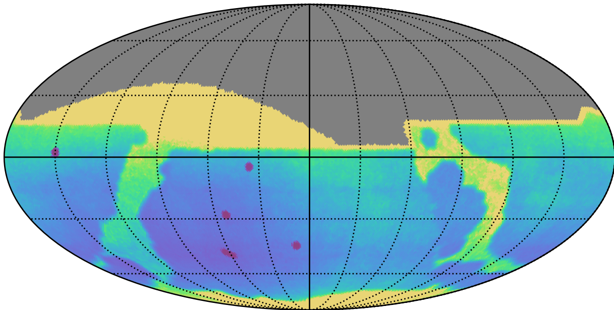
early_u_fpextra2.0_v3.4_10yrs All sky: Parallax Uncert @ 22.4
