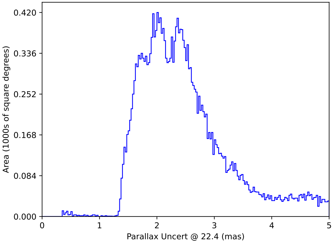
early_u_fpextra2.0_v3.4_10yrs All sky: Parallax Uncert @ 22.4
