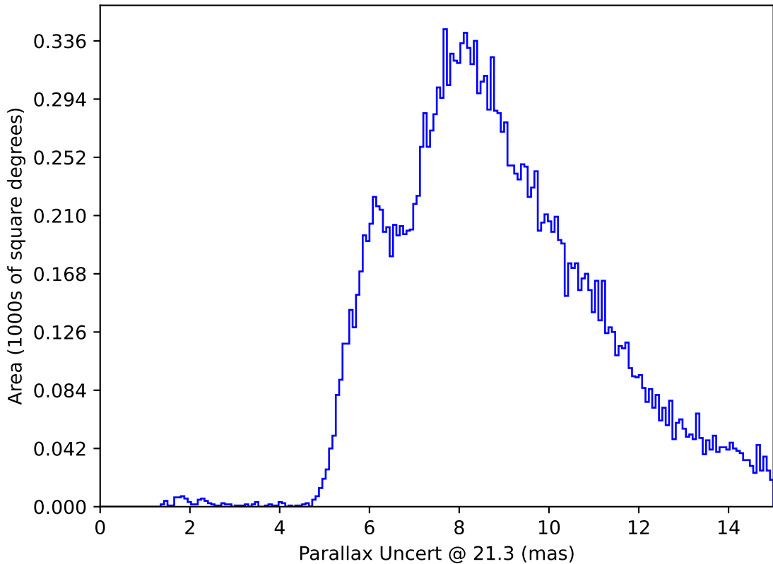
early_u_fpextra2.0_v3.4_10yrs All sky y band only: Parallax Uncert @ 21.3
